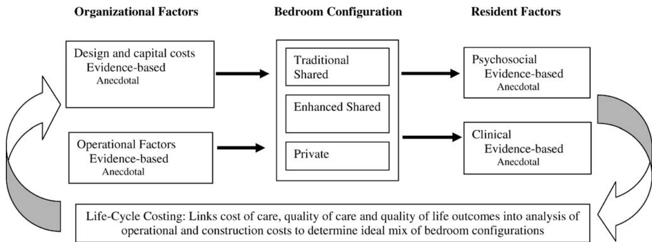
Figure 1. Conceptual framework.
